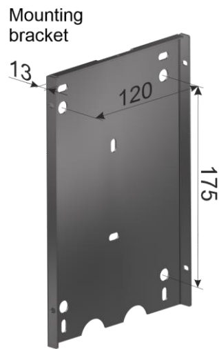
Fig.5 - Mounting bracket for charging station installation Fig.6 - Possibility of power cable routing from the rear side of the charging station
