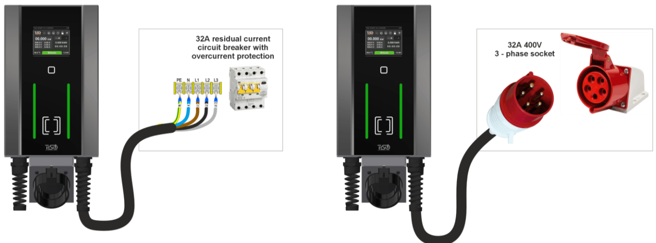
Fig. 9 - Three-phase charging station connection options
