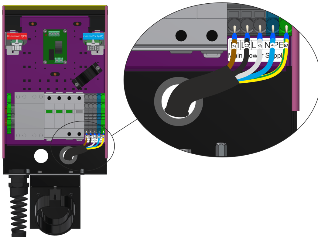
Fig. 12 – Connecting the power cable
