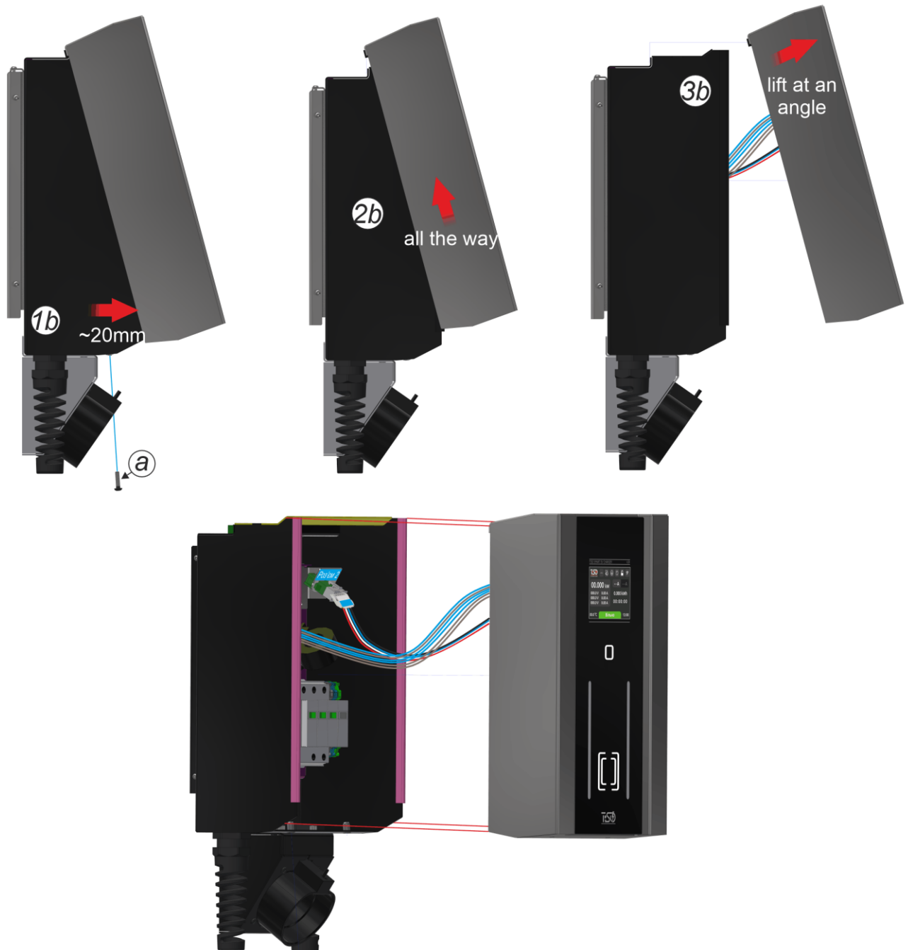
Fig. 10 – Removing the front cover of the charging station
