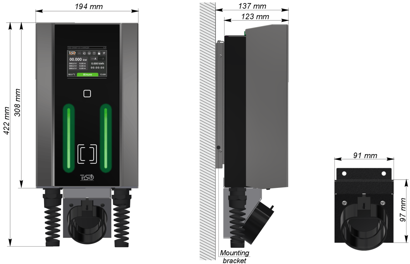
Fig. 3 - Overall dimensions of the EV charging station
