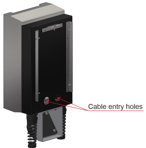
Fig.5 - Mounting bracket for charging station installation Fig.6 - Possibility of power cable routing from the rear side of the charging station
