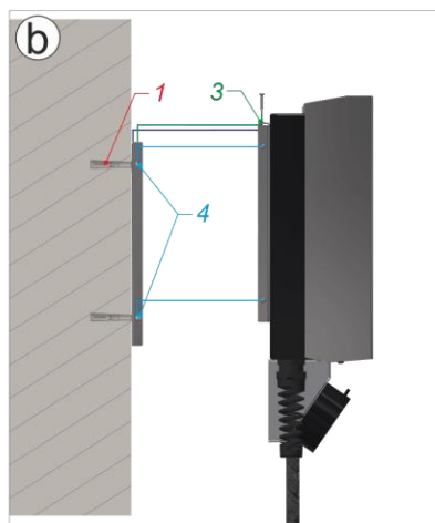
Fig.7 – Step-by-step wall mounting
