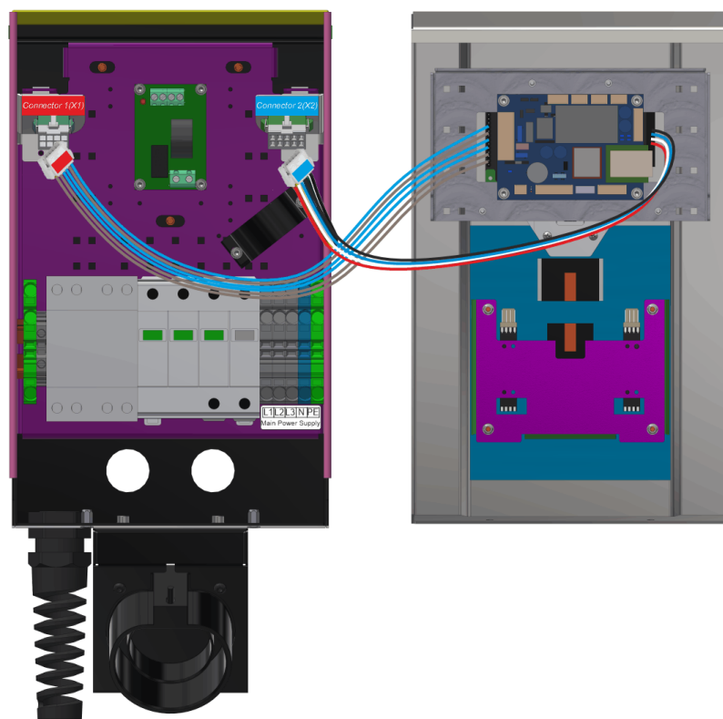
Fig. 11 – Disconnecting Mini-Fit connectors
