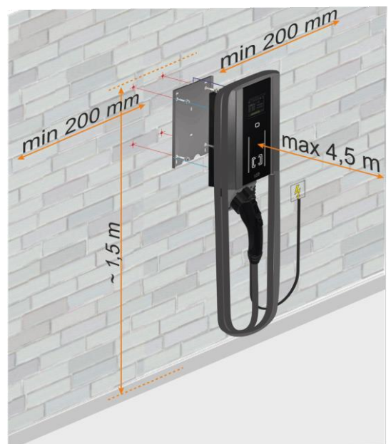
Fig.4 – Wall mounting
